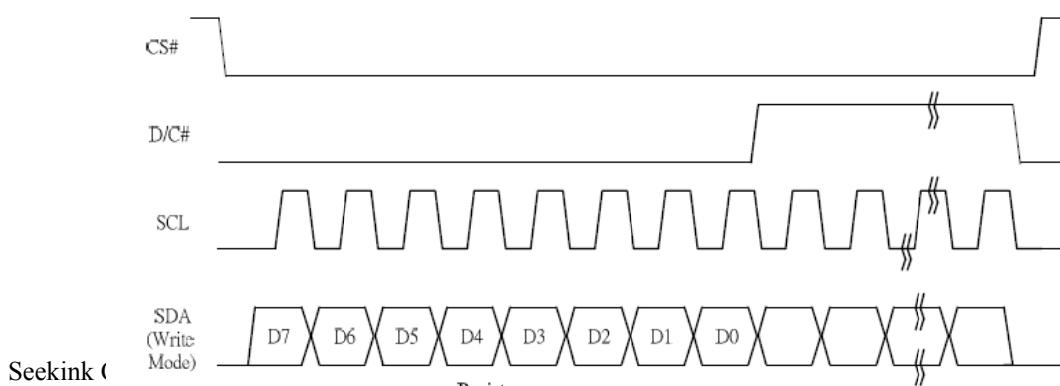
Figure 7-1 Write procedure in 4-wire SPI mode
